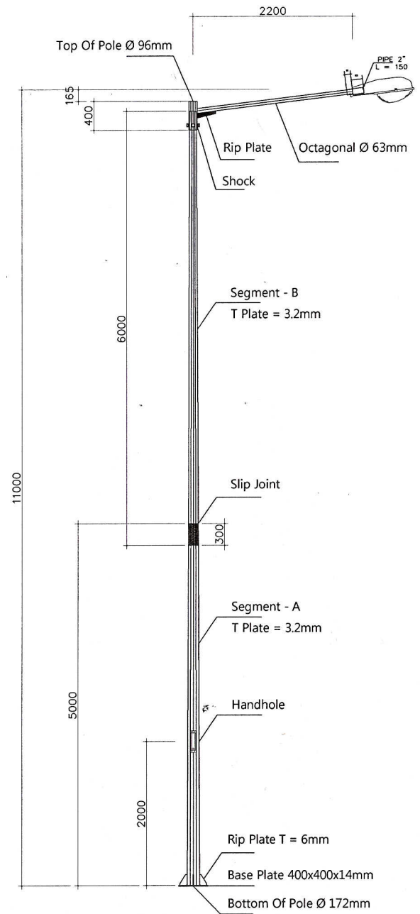
Tiang PJU H-11 M Single T SCALE 1 : 25 OCTAGONAL
