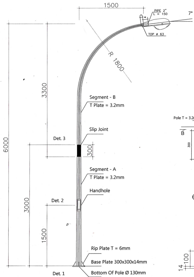
TIANG PJU H-06M SINGLE PARABOLE SCALE 1 : 25 OCTAGONAL
