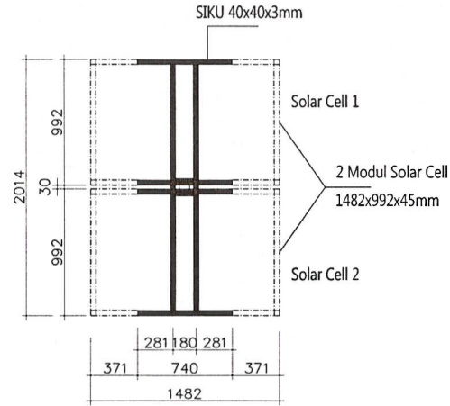
Det 3. Bracket Modul Solar Cell SCALE 1 : 25
