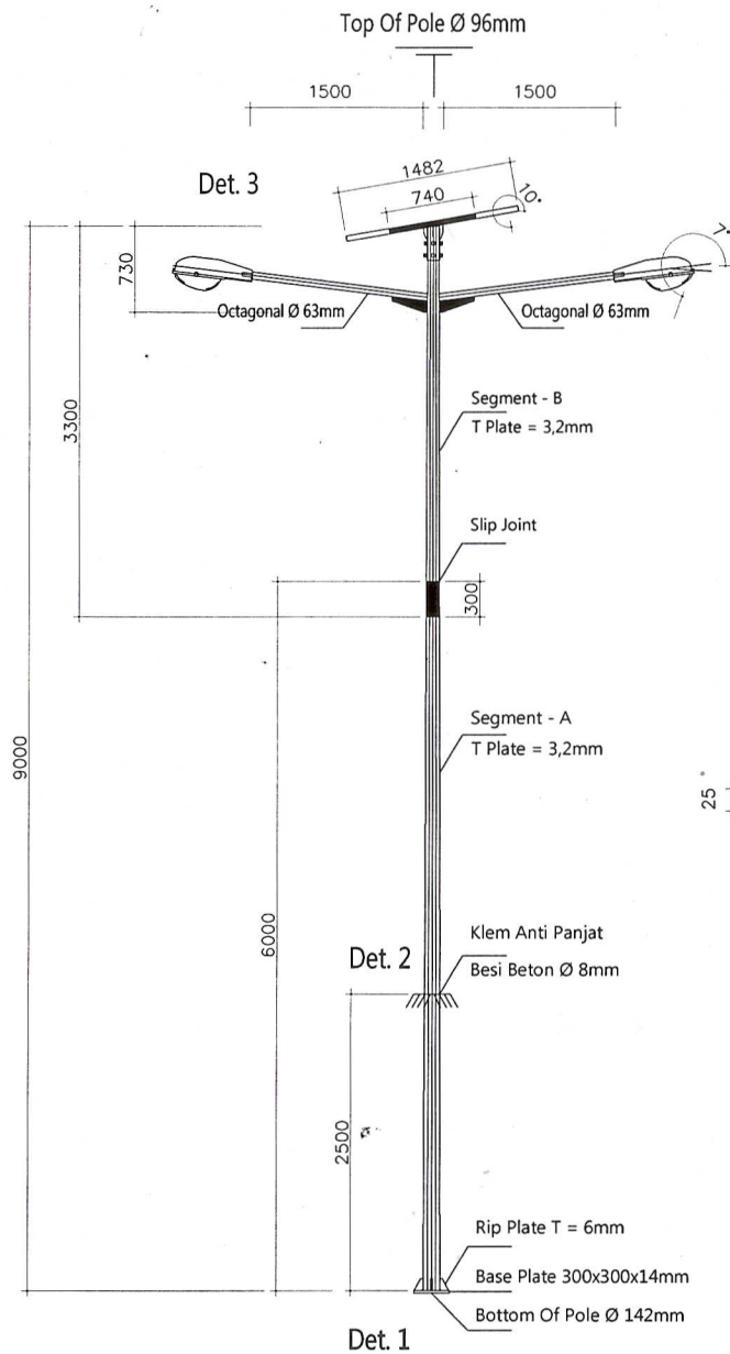
TIANG PJU H-09M DT TYPE SC SCALE 1 : 100
