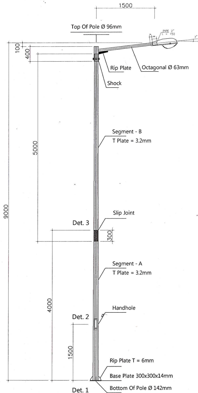
Tiang PJU H-09 M Single T SCALE 1 : 25 OCTAGONAL
