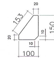
DET 1. RIP PLATE SCALE 1 : 25
