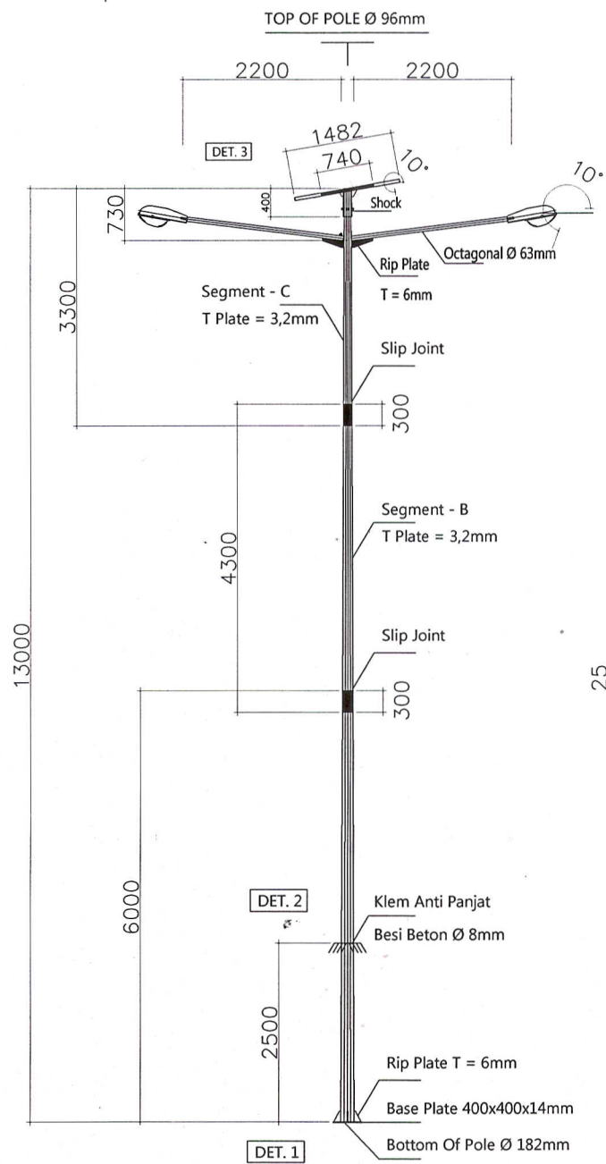
TIANG PJU H-13M DT TYPE SC SCALE 1 : 100
