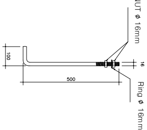
Det Anchor Bolt SCALE 1 : 25
