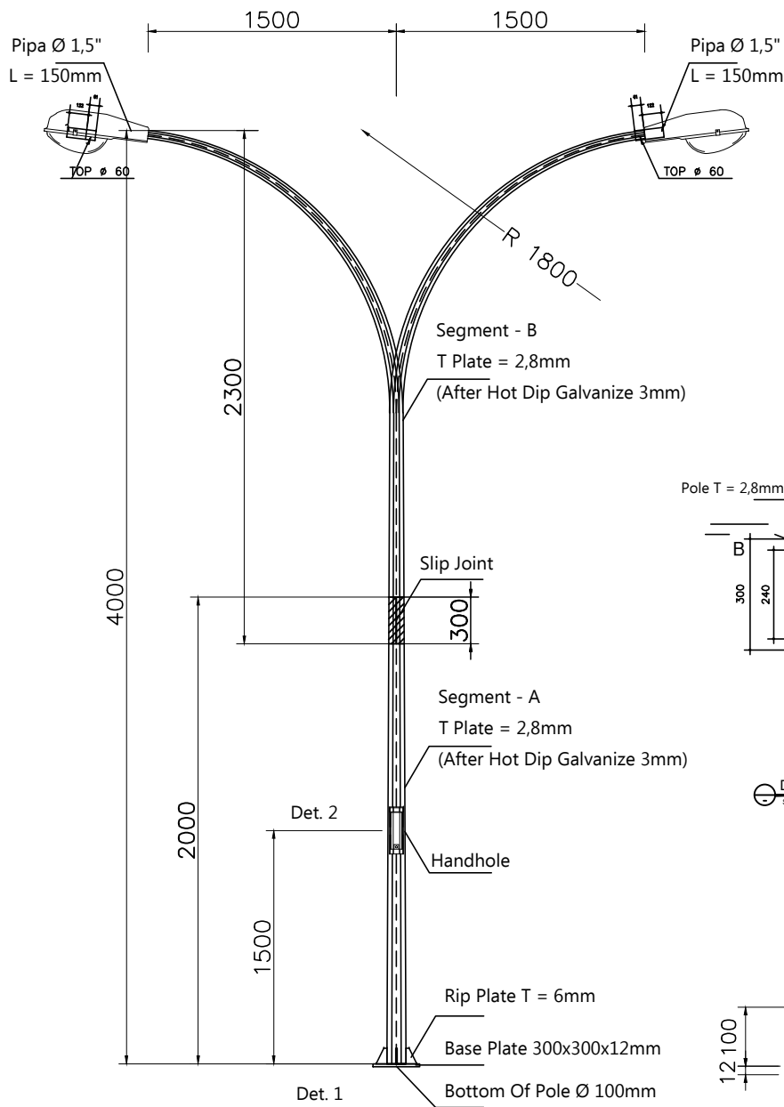
TIANG PJU H-04M DOUBLE PARABOLE SCALE 1 : 25 OCTAGONAL
