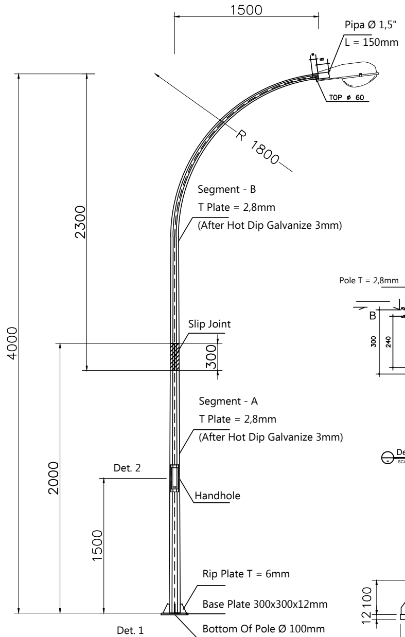
TIANG PJU H-04M SINGLE PARABOLE SCALE 1 : 25 OCTAGONAL
